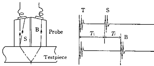
Fig. 2 Auto zero adjustment (T: Transmitted pulse S: Surface reflected echo T_1 : Thickness of material measured T_2 : Time required for reciprocation)
